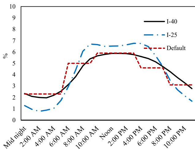
Fig. 5 Hourly Truck Distribution
