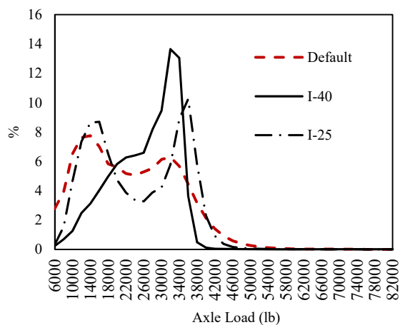
(b) Tandem axle
