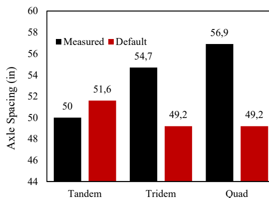
Fig. 8 Average axle spacing
