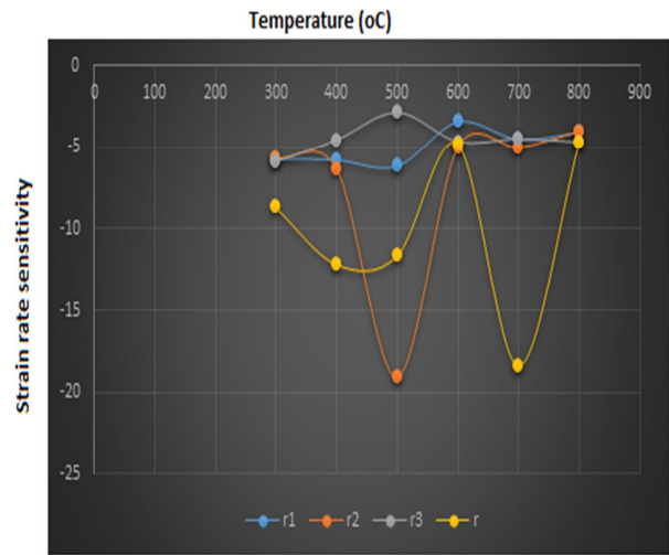
Fig. 2 Variation of (SRS) with Temperature at six temperatures within the negative SRS range for grain size variants
