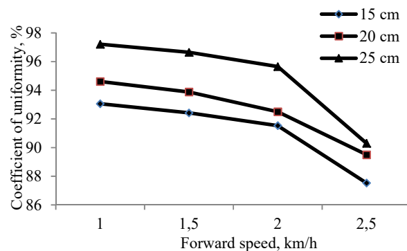
Fig. 2 Coefficient of uniformity as affected by forward speed
