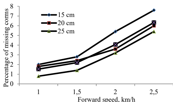
Fig. 3 Missing as affected by speed of operation
