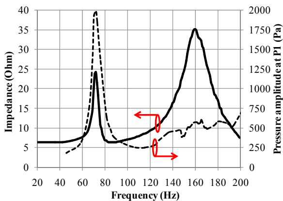
Fig. 4 Loudspeaker impedance and pressure curves
