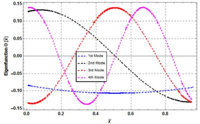
Fig. 7 The Plot of Eigenfunctions against the Dimensionless Displacement for the First Four Modes when the Number of Elements, N=100
