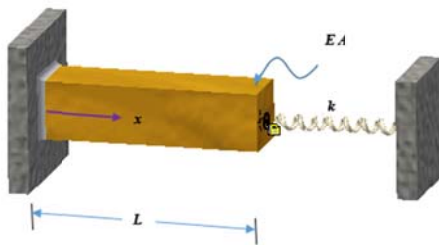
Fig. 2 Cantilever with Fixed Spring
