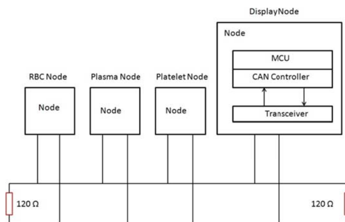
Fig. 2 CAN Bus Block Diagram
