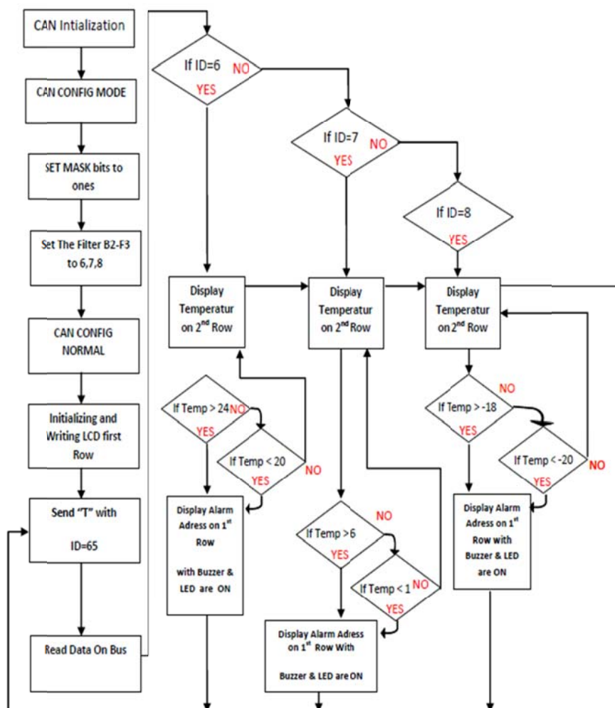
Fig. 7 Flow Chart For CAN Based Display Node
