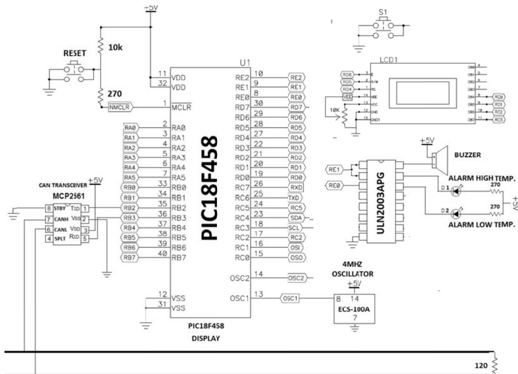
Fig. 6 Display Node Schematic Diagram
