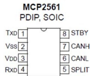
Fig. 1 CAN Transceiver
