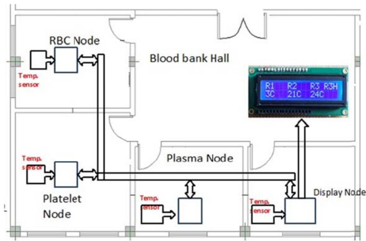
Fig. 5 Blood Bank Center designed layout
