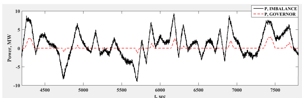
Fig. 5 Power generation by Governor
