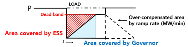
Fig. 2 The proposed model for ESS PFR service
