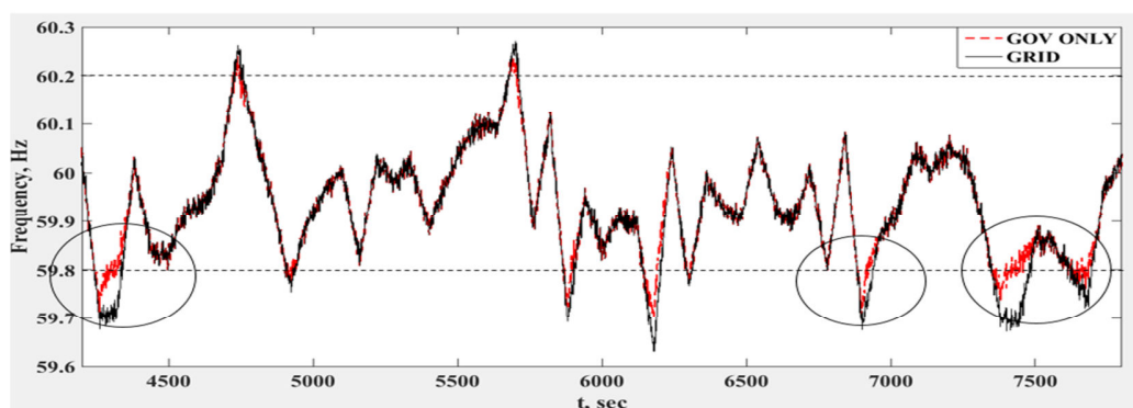
(a) Frequency regulation by Governor
