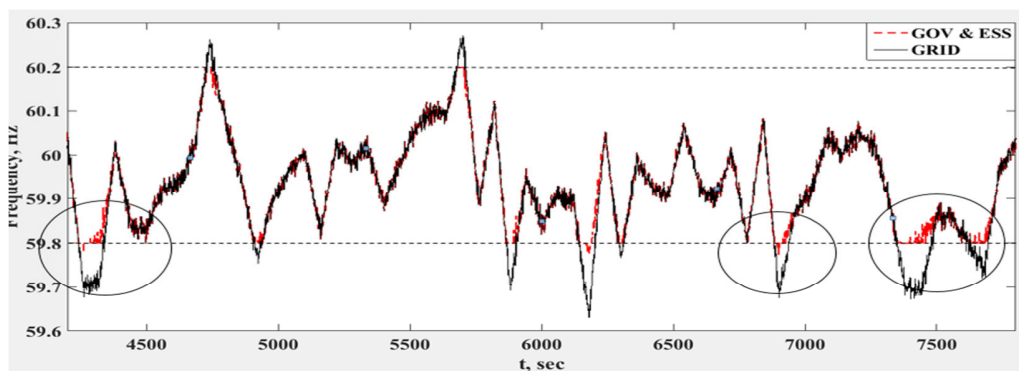
(b) Frequency regulation by ESS and Governor
