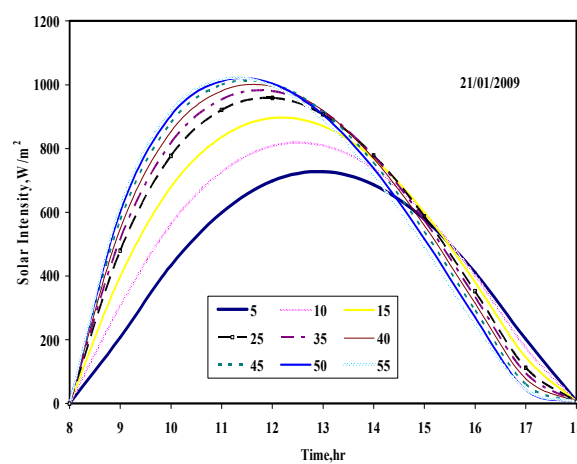
Fig. 19 Effect of the collector tilt angle on the solar radiation unit in summer
