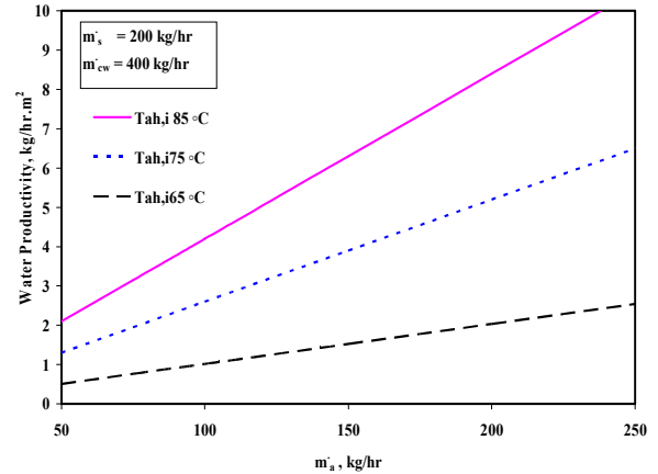
Fig. 14 Variation of feed water flow rate and temperature on water productivity along an operating day
