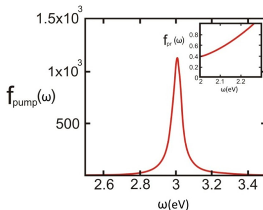
Fig. 2 Dependence of internal field enhancement of the pump wave frequency for SC in the medium with n = 1.6 . The inset shows the same for the probe wave
