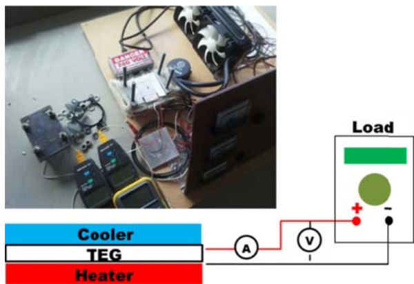
Fig. 3 The single cell TEG testing layout
