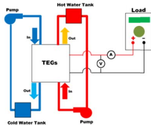
Fig. 8 System schematic
