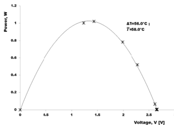
Fig. 5 Power-voltage curve for single TEG
