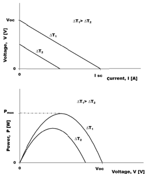
Fig. 2 Typical voltage-current and power-voltage curve for TEG
