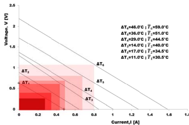
Fig. 6 Voltage-current graphs with different temperature difference
