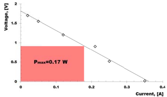
Fig. 12 Testing result
