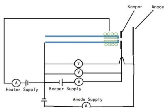
Fig. 3 Test apparatus for discharge cathode life test
