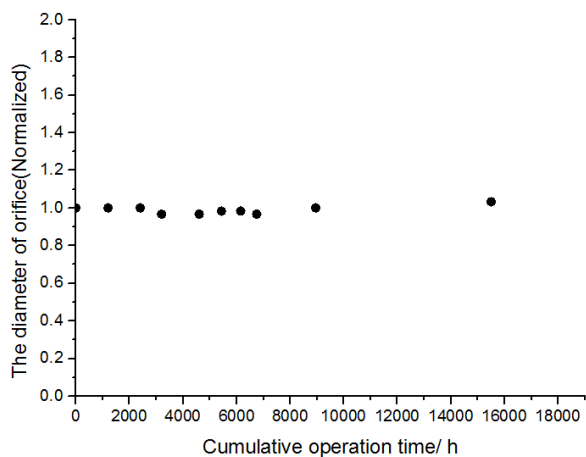
Fig. 7 The diameter of orifice versus operation time
