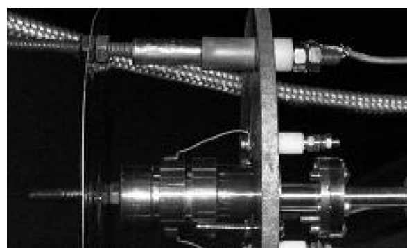
Fig. 4 The hollow cathode heater test platform
