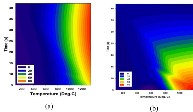
Fig. 6 Propagation of cooling rate along the longitudinal direction from the fusion boundary at z = 36 mm (a) SMAW and (b) GTAW
