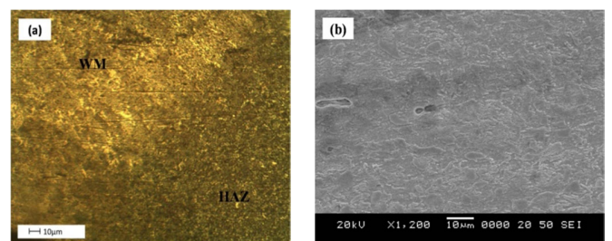
Fig. 11 Microstructural morphology of heat affected zone of welded joint by GTAW (a) Optical micrograph (OM) and (b) Scanning electron micrograph (SEM)
