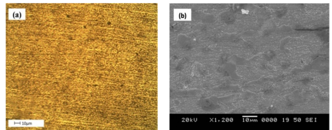
Fig. 10 Microstructural morphology of base metal of welded joint by GTAW (a) Optical micrograph (OM) and (b) Scanning electron micrograph (SEM)
