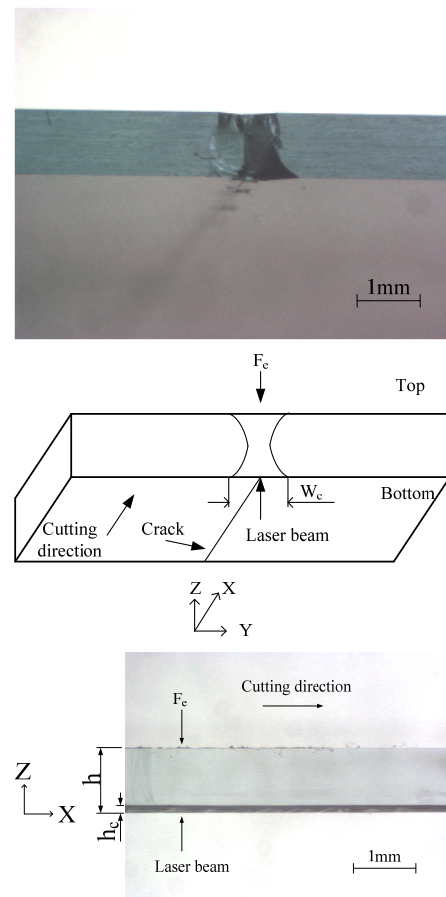
Fig. 16 Definitions of the crack contours
