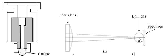
Fig. 2 Lens system for the laser thermal cleavage with a contact ball-lens
