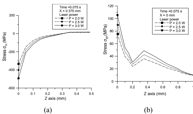
Fig. 11 Distributions of the normal stress \sigma_{yy} along z axis at the beam center and behind the beam center at x=0.375 mm with variable laser powers.
