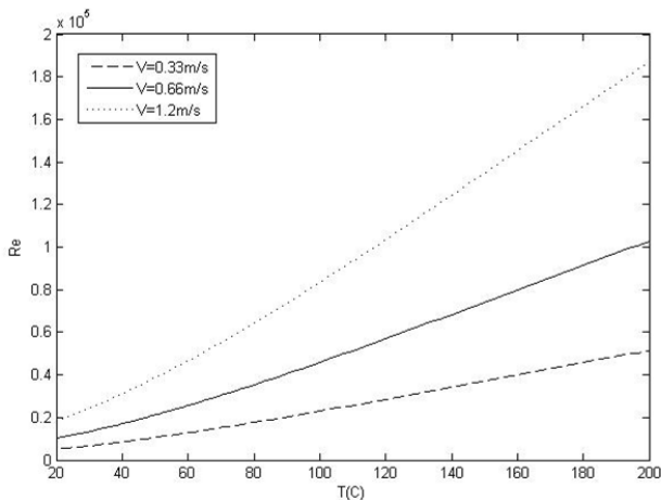
Fig. 3 Reynolds vs oil temperature graph for various types of oil velocities
