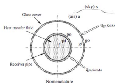
Fig. 1 Collector receiver model of nomenclature
