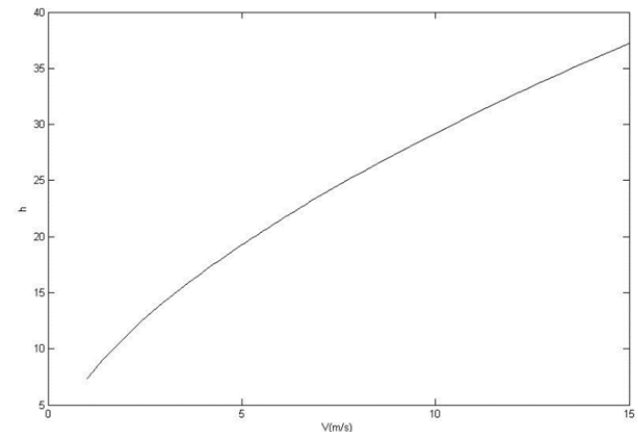
Fig. 9 Convection coefficient vs wind velocity graph at T=40C
