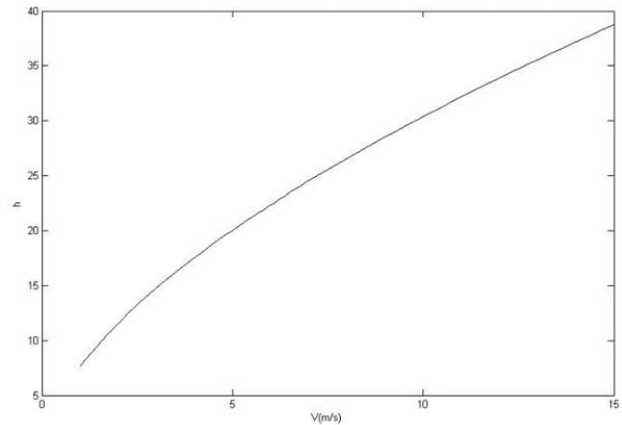
Fig. 8 Convection coefficient vs wind velocity graph at T=10C
