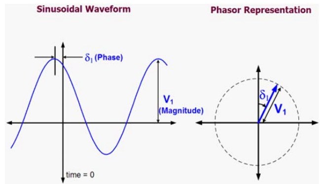
Fig. 1 Sinusoid and its corresponding phasor representation
