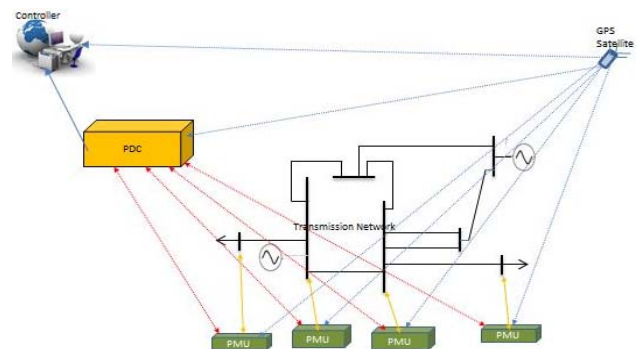
Fig. 2 Synchrophasor architecture
