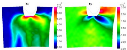
(c) Loading = 22.10kN
