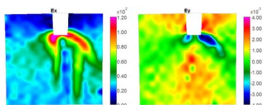
(a) Loading = 14.43 kN
