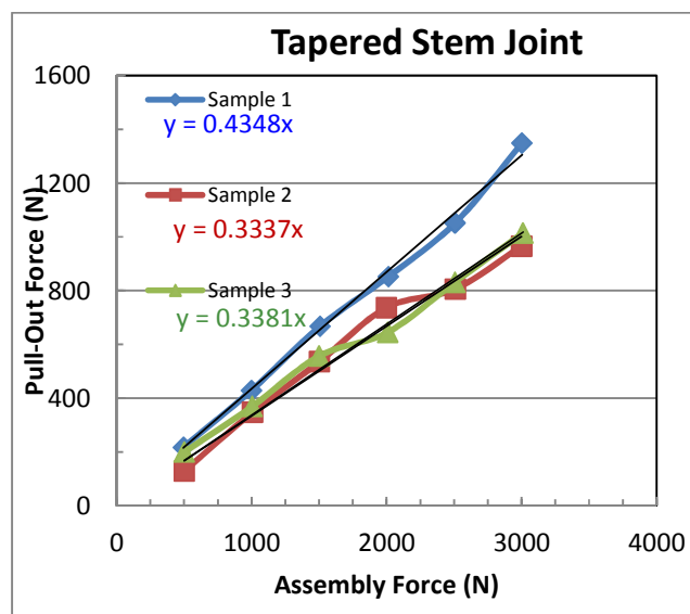
Fig. 7 Pull-out forces achieved for the three samples for the tapered stems depending on different assembly forces
