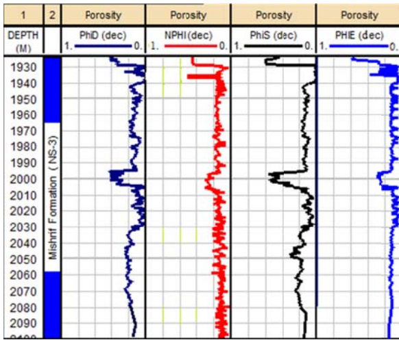
Fig. 2 Porosity results
