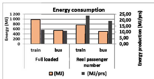
Fig. 4 Evaluation of the energy consumption
