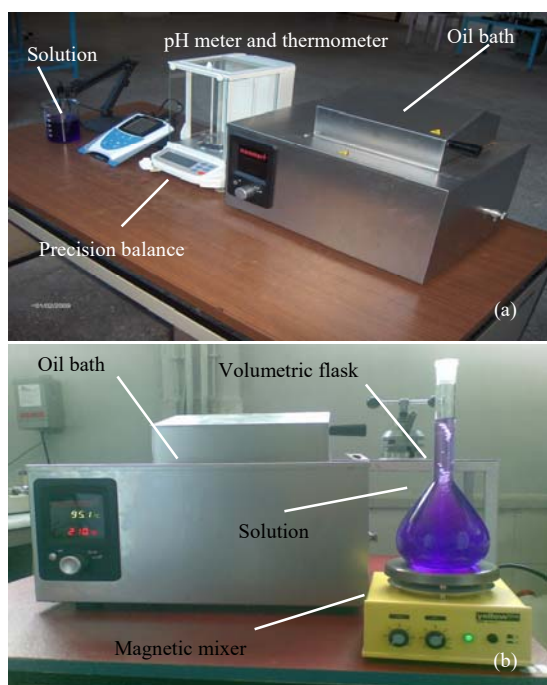
Fig. 2 The equipment for electroless Ni-B deposition
