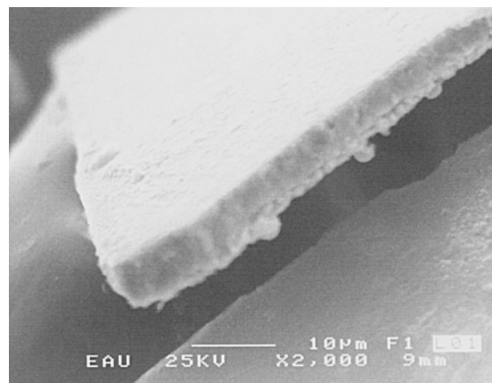
Fig. 4 Cross-sectional SEM image of electroless Ni-B coating
