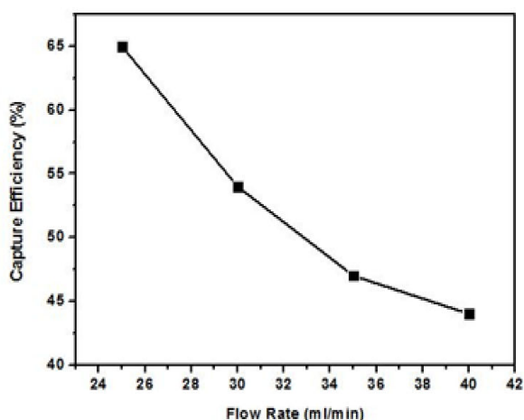
Fig. 4 Capture efficiency versus flow rate curve of Fe_3O_4 nanoparticles of an implant assisted channel at different flow rates (25-40 ml/min)
