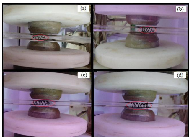
Fig. 1 Images of captured \text{Fe}_3\text{O}_4 nanoparticles at different magnetic fields: (a) 2, (b) 3, (c) 4 and (d) 5 kG at particle concentration 0.6mg/ml and at flow rate 30 ml/min in an implant assisted channel
