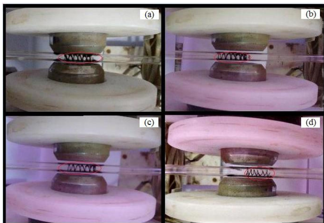
Fig. 3 Images of captured Fe_3O_4 nanoparticles at different flow rates: (a) 25, (b) 30, (c) 35 and (d) 40 ml/min at particle concentration 0.6 mg/ml and at magnetic field 3kG in an implant assisted channel
