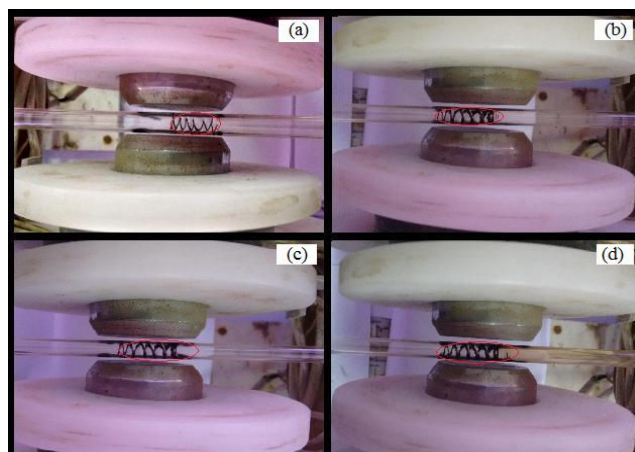
Fig. 5 Image of captured Fe_3O_4 nanoparticles at different particle concentration: (a) 0.3, (b) 0.4, (c) 0.5, and (d) 0.6 mg/ml at flow rate 30 mg/ml and at magnetic field 3kG in an implant assisted channel
