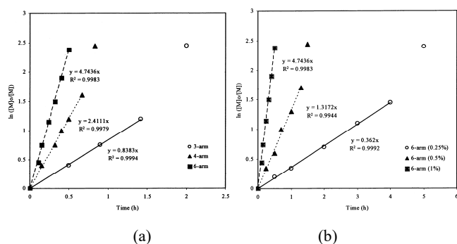
Fig. 4 Kinetic plots of \ln([M]_0/[M]) vs. time for the polymerization of t-BA: (a) Initiation with 3-, 4- and 6-arm initiators: initiator/t-BA = 1% (by mole); (b) Initiation with 0.25%, 0.5% and 1% of 6-arm initiator/t-BA
