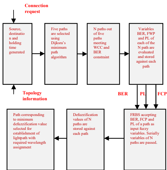
Fig. 9 Block diagram of execution of a connection request using proposed algorithm FWM-aware FDRWA
