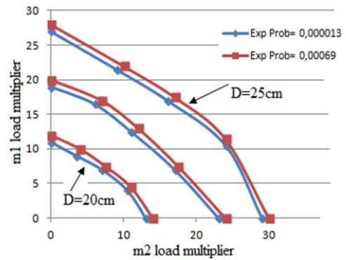
Fig. 7 Safe loading domain for plastic limit design
