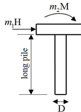
Fig. 9 Loads on the fixed-head pile
