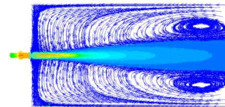
Fig. 7 The vector figure of the Y type jet atomizer at the y=0 face
