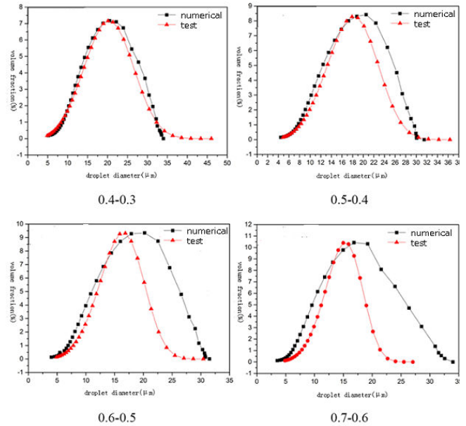
Fig. 11 The distribution of the volume fraction
