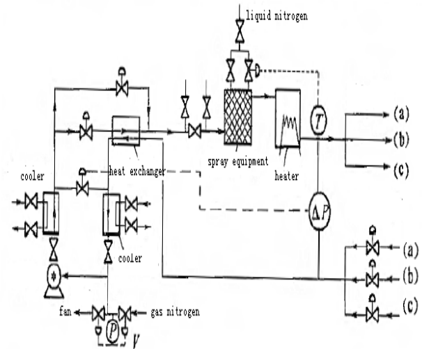
Fig. 1 Flowchart of the temperature regulating system by gaseous nitrogen
