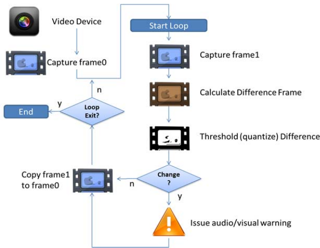
Fig. 1 Change detection Algorithm
