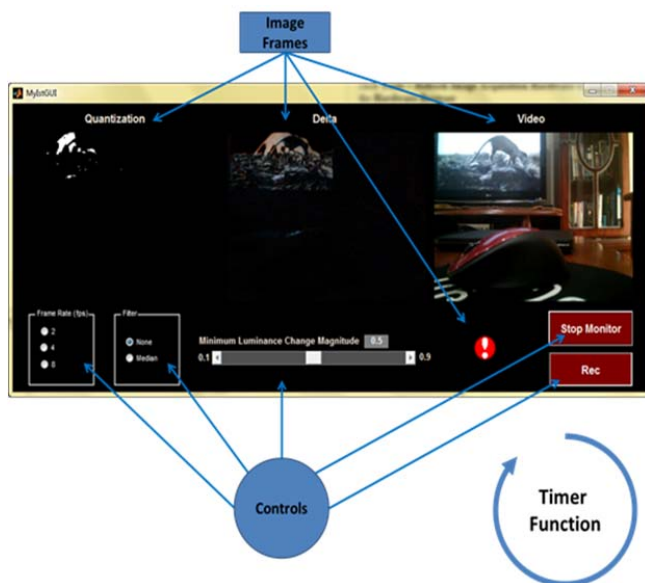
Fig. 4 System's GUI
