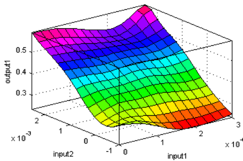
Fig. 5 The rule surface view
