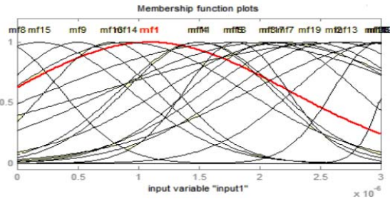
Fig. 4 The membership functions for input variable
