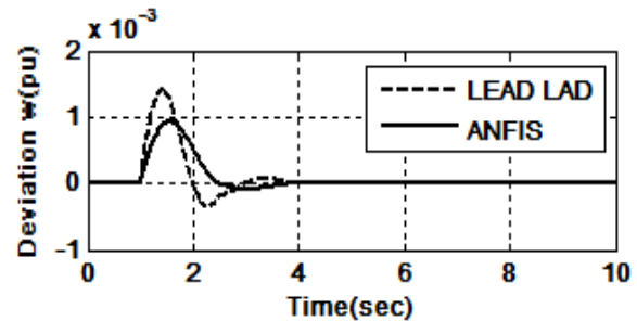
Fig. 8 Angular Velocity deviations during step change in Mechanical input power for nominal load ( \delta_1 controller)
