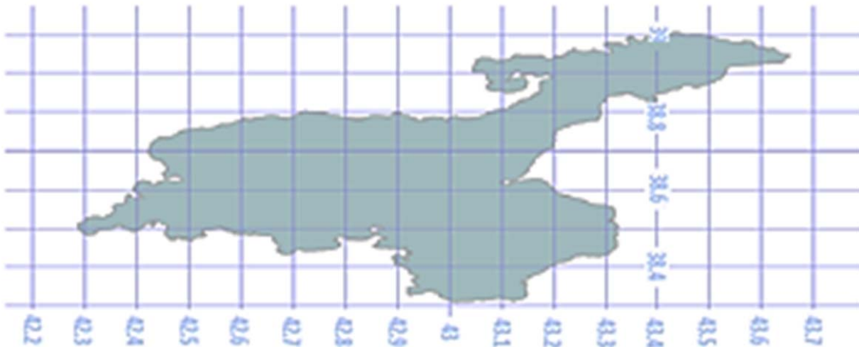
Fig. 2 Location information of Lake Van
