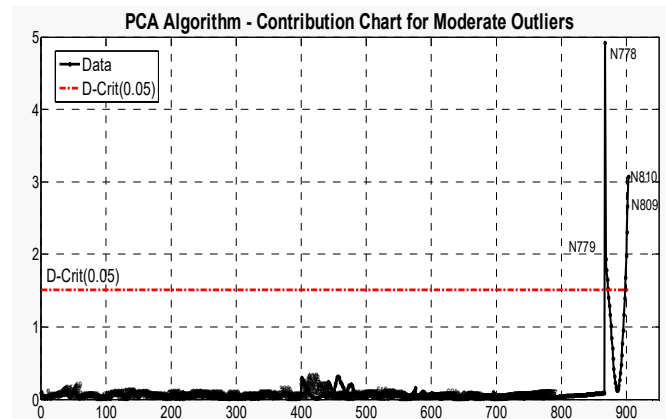
Fig. 10 PCA algorithm contribution plot
