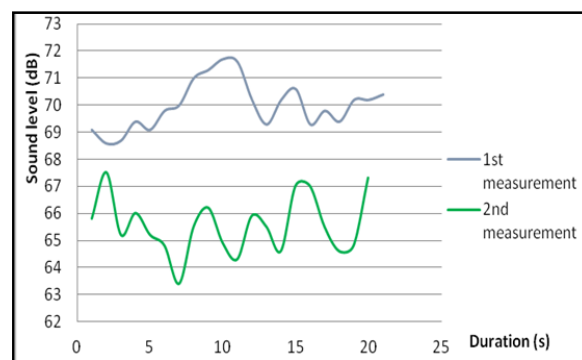
Fig. 4 Sound level in Citroen Berlingo during acceleration
