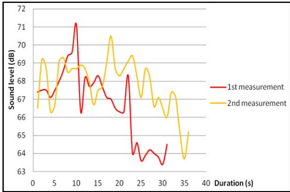
Fig. 5 Sound level in Jaguar X-type during acceleration
