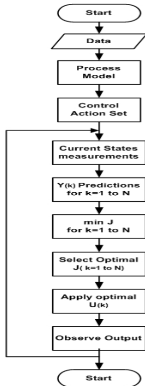
Fig. 6 MPC algorithm
