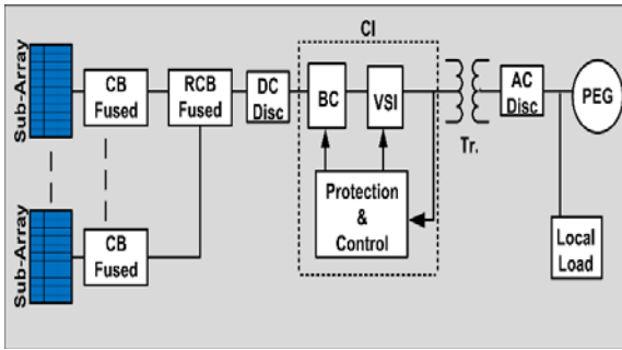
Fig. 1 PV System
