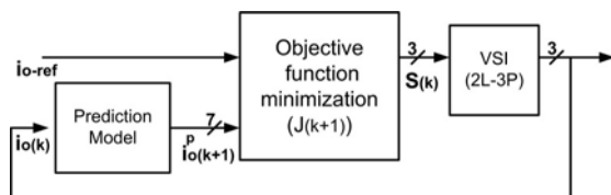
Fig. 5 VSI MPC control block diagram
