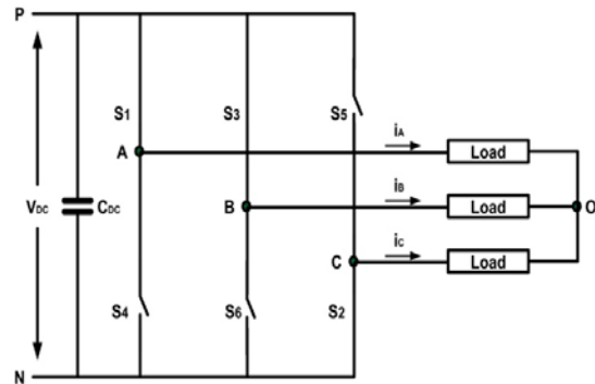
Fig. 4 VSI circuit for S_1S_2S_3=111
