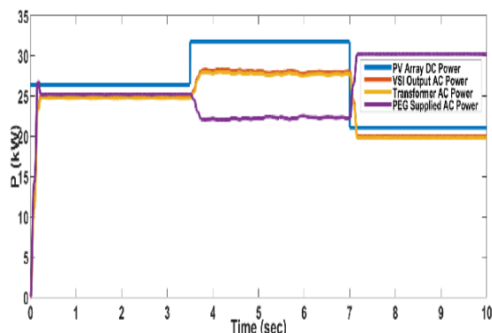
Fig. 7 Power Graphs
