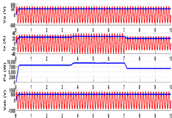
Fig. 9 V_s and i_s at varying P
