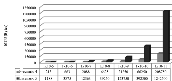
Fig. 5 DOCSIS 3.0 with EHDR Vs DOCSIS 3.0 without EHDR
