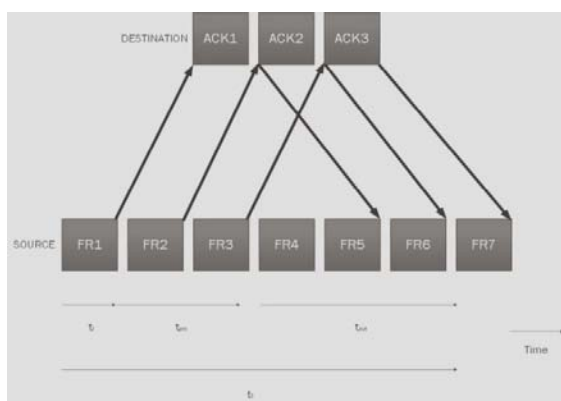
Fig. 3 Continuous transmission of frames [29]
