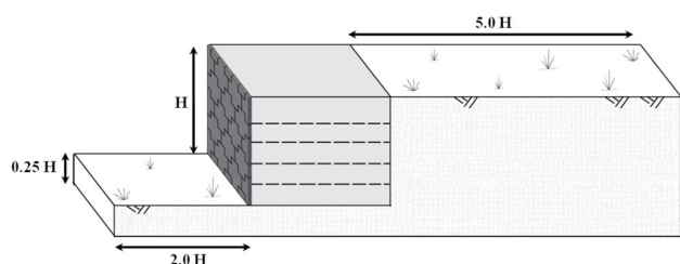
Fig. 3 Dimensions of fabricated models
