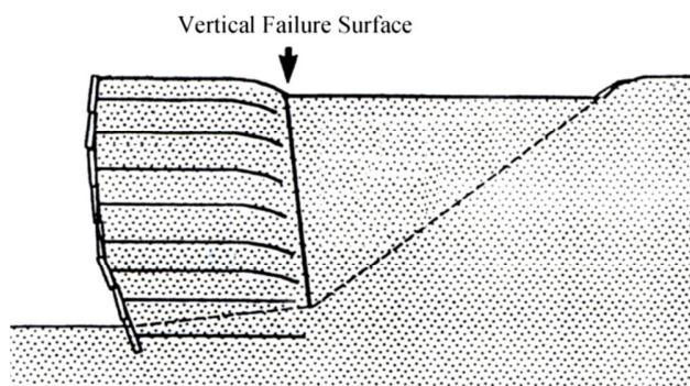
Fig. 2 Fracture surfaces in centrifugal tests
