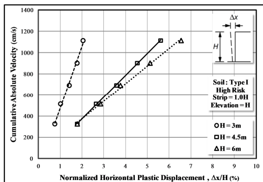
Fig. 11 Optimal convergence between CAV and residual displacements
