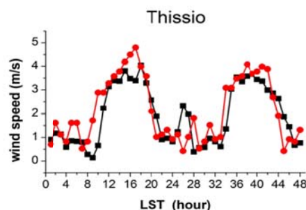
Fig. 6 Comparison of the modeled (black line) and measured (red line) wind speeds at the NOA station
