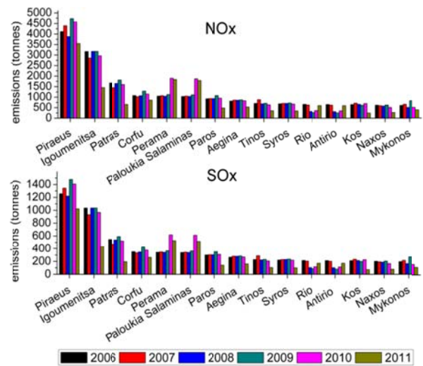
Fig. 4 Annual emission of pollutants from SNAP category 7
