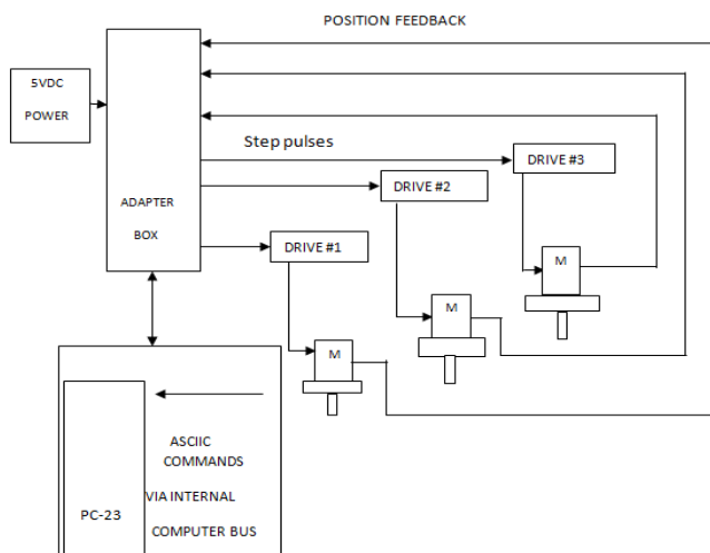
Fig. 3 Schematic of the FDM control process
