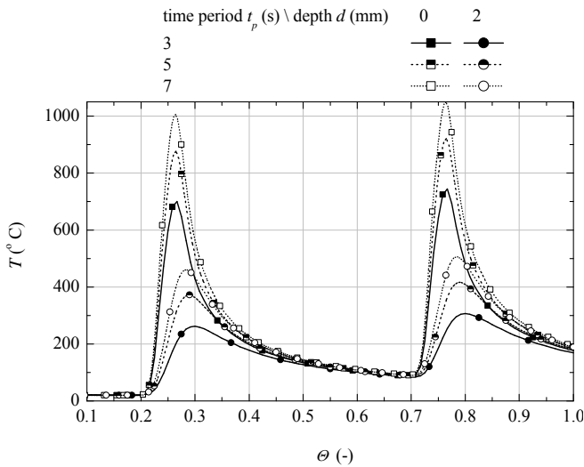
Fig. 6 Time courses of the temperature in the center of sample front surface for depths 0 and 2 mm ( x = 50 mm, y = 35 mm)
