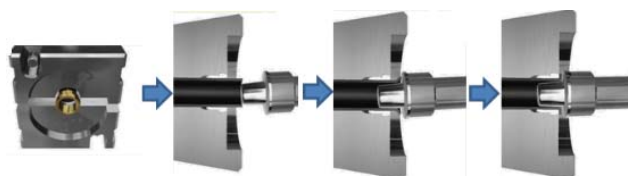
Fig. 2 Orbital-forming process
