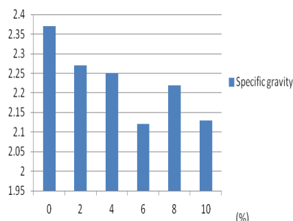
Fig. 4 Specific gravity against percentage replacement
