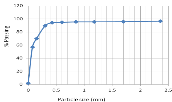
Fig. 3 Particle size distribution of untreated lateritic soil
