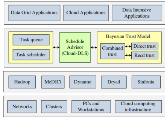
Fig. 1 Trusted dynamic scheduling framework
