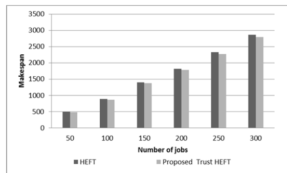
Fig. 2 Makespan Achieved
