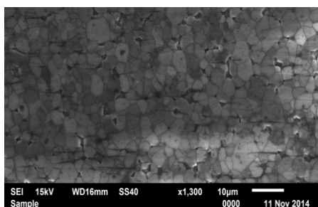
Fig. 5 Micrographs of ceramic composites obtained at 1600°C ( \text{Al}_2\text{O}_3 - \text{ZrO}_2 -MgO)
