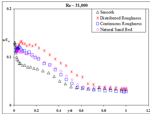
Fig. 4 Streamwise turbulence intensity for flow over different bed condition
