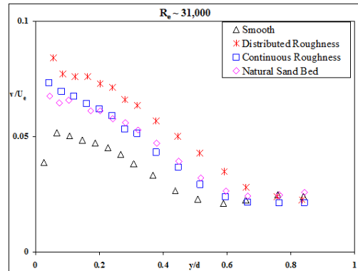
Fig. 5 Vertical turbulence intensity for flow over different bed condition
