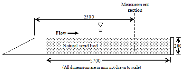
Fig. 3 Section of natural sand bed
