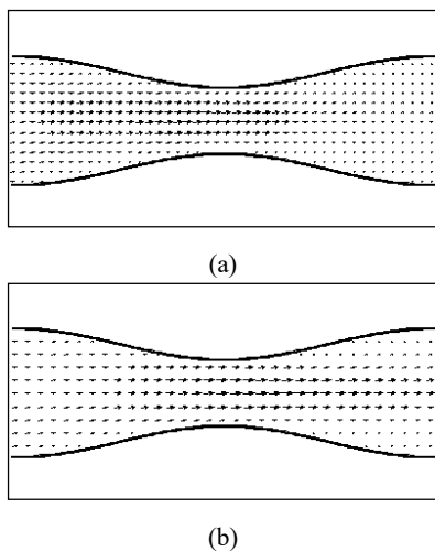
Fig. 4 Velocity vector plot for (a) case I and (b) case III
