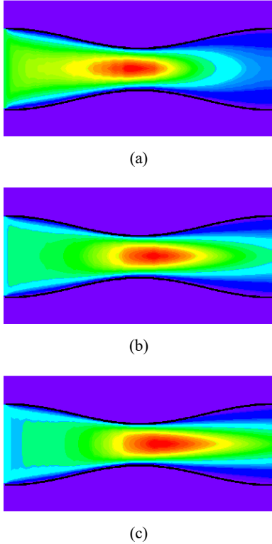
Fig. 3 Axial velocity distribution for (a) case I, (b) case II, and (c) case III
