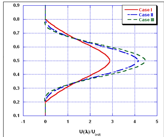
Fig. 6 Velocity profiles at the end-section of the wave for the different cases considered
