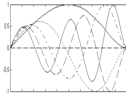
Fig. 6 The lowest five mode shapes for a non uniform S-C beam for r=0.5
