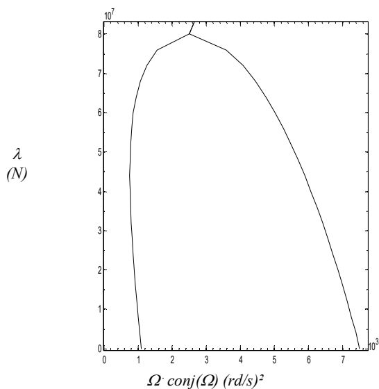
Fig. 17 The load-frequency curve for a non uniform slender C-F beam for r=0.1 , \lambda f=8.7 \times 10^7 N
