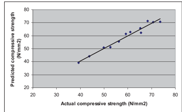
Fig. 4 Actual compressive strength versus predicted compressive strength at 365 days using linear regression model
