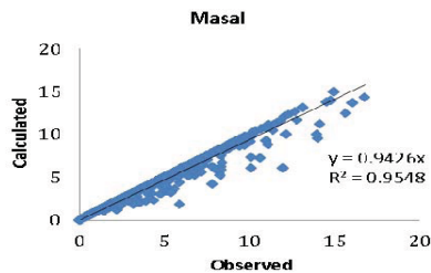
(f) Masal River outflow comparison
