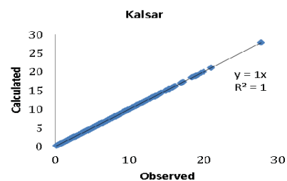
(c) Kalsar River outflow comparison
