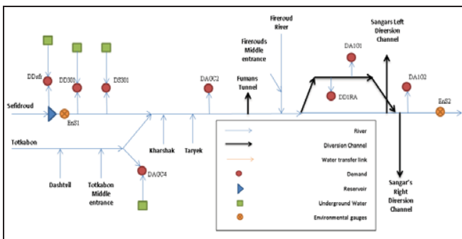
Fig. 2 Node-link schematic view of Sefidroud River system
