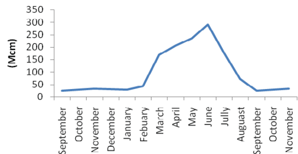
Fig. 6 Sefidroud's reservoir monthly average rule curve
