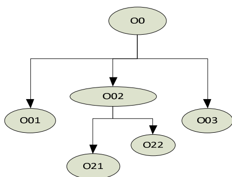
Fig. 2 Ontology Hierarchy
