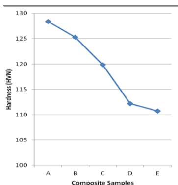
Fig. 2 Variation in Hardness for ZA-27/ Al_2O_3 -Cg and ZA-27/ Al_2O_3 -FA-Cg Reinforced Composite Samples
