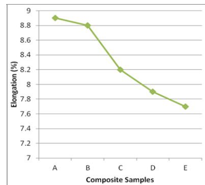
Fig. 4 Variation in percentage elongation for ZA-27/ Al_2O_3 -Cg and ZA-27/ Al_2O_3 -FA-Cg reinforced composite samples
