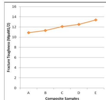
Fig. 5 Variation in fracture toughness for ZA-27/ Al_2O_3 -Cg and ZA-27/ Al_2O_3 -FA-Cg reinforced composite samples
