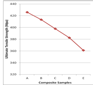
Fig. 3 Variation in ultimate tensile strength for ZA-27/ Al_2O_3 -Cg and ZA-27/ Al_2O_3 -FA-Cg reinforced composite samples
