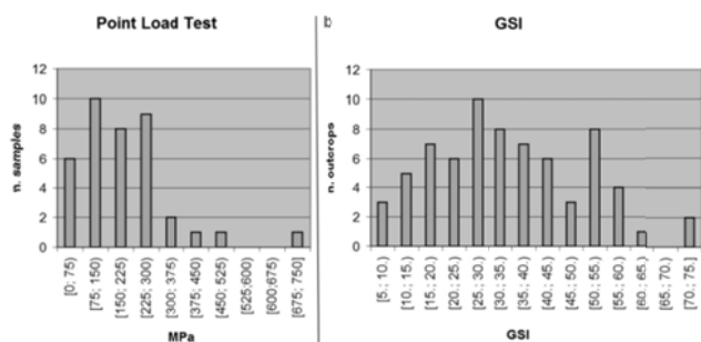
Fig. 6 Distribution of: (a) compressive strength perpendicular to the schistosity, (b) Geological Strength Index in each outcrop (Fig. 4)
