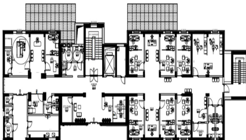
Fig. 7 Floor Plan after Strengthening the Load-Bearing System of the Building
