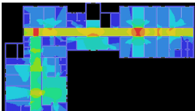
Fig. 13 Connectivity values before change (2066)
