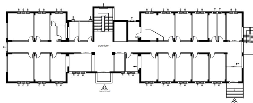
Fig. 5 Ground floor plan of the building before change
