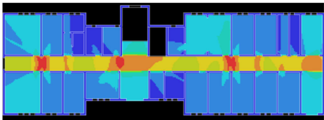
Fig. 12 Connectivity values before change (1800)
