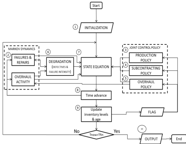
Fig. 4 Simulation model block diagram
