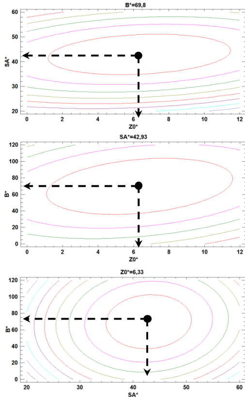
Fig. 6 Contours of the estimated response surface
