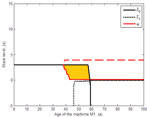
Fig. 5 Control parameters approximation
